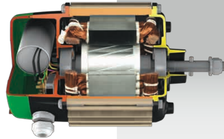
In-house motor production with qualitative advantages for variable speed fans.
